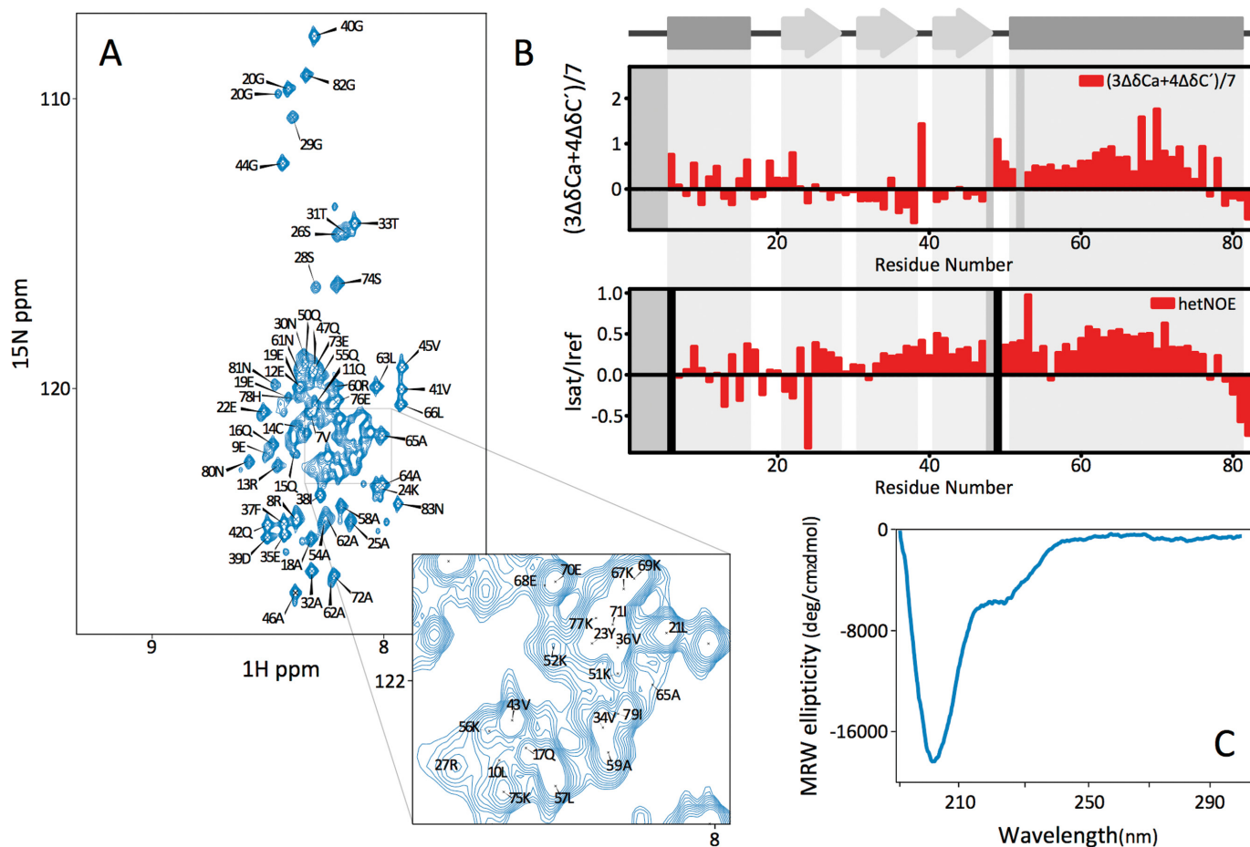
Figure 2. Spectroscopic characterization of the free unfolded form of DCL1-A. (A) ^1\text{H} - ^{15}\text{N} -HMQC spectrum. (B) Combined CA and C' secondary chemical shifts (top) and ^1\text{H} - ^{15}\text{N} heteronuclear NOEs (bottom). Secondary structure elements of the folded form are schematized on top. Vertical black bars indicate Pro residues and gray bars indicate unassigned resonances. (C) UV-CD spectrum.
