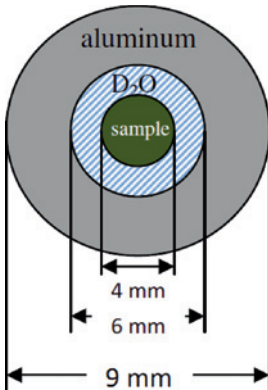
Figure 1: View from the top of the experimental setup of the cylindrical high pressure container. The container is built of a high-tensile aluminum alloy; it is filled with an aluminum cartridge containing the sample and with D_2O .
