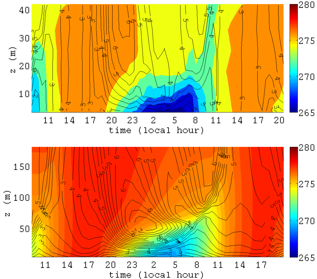
FIGURE 8 – Potential temperature and wind speed isocontours from tower observations (top) and in the 180 first meters of the simulation (bottom). Potential temperature, calculated with a reference level at 1013 hPa, ranges so "high" above 0 °C due to the elevated altitude of Dome C and the associated low pressure ( \sim 650 hPa). Corresponding absolute temperature is of about -30 °C.
