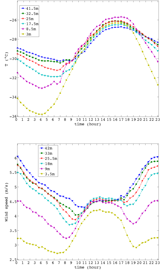
FIGURE 4 – Mean diurnal cycle in temperature and wind speed. Night-time December data from 2009 to 2011.
