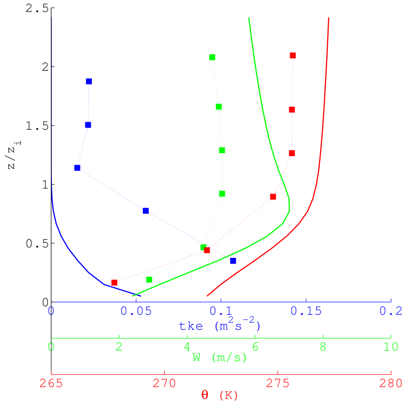
FIGURE 12 – Vertical profiles of potential temperature, wind speed and turbulent kinetic energy. Data are shown at midnight. Observational data from the tower are shown by the square; simulation results are represented by the solid line. The vertical scale is normalized with the ground-base inversion layer depth (20 m in the observational data and 60 m in the simulation).
