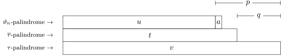
Figure 1: Illustration of the proof of Lemma 24.
