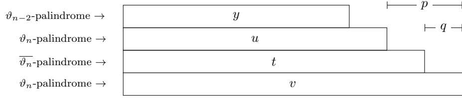
Figure 2: Illustration of Part ( \Leftarrow ) in the proof of Proposition 26. It follows from Lemma 24 that p = 2g and q = g , where g = \gcd(p, q) . Also, \vartheta_{n-1} = \vartheta_n .
