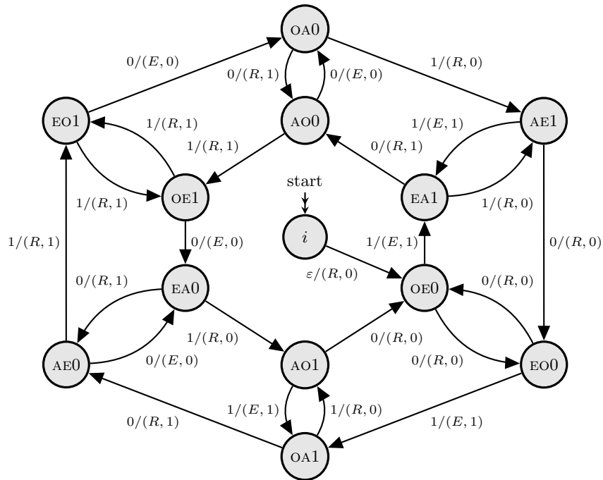
Figure 4: Transducer computing the directive bi-sequence of a Rote standard word \mathbf{r} starting with 0 from the directive sequence of a Sturmian standard word \mathbf{s} such that \Delta(\mathbf{r}) = \mathbf{s} .
