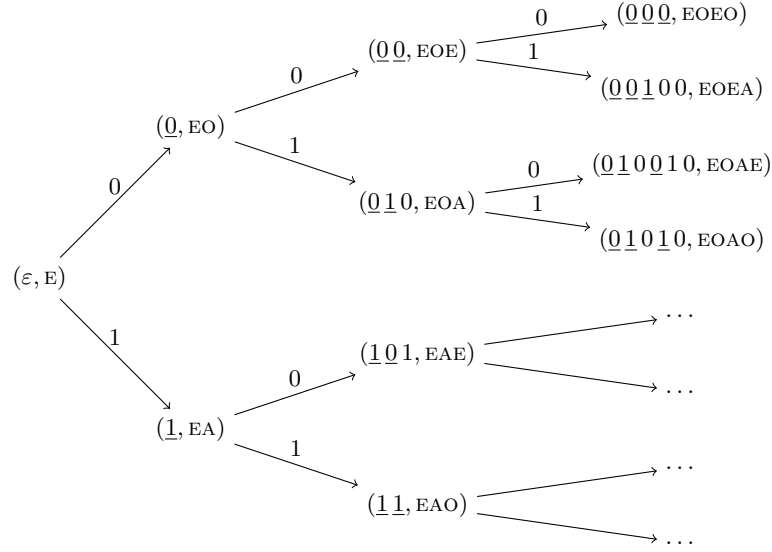
Figure 3: Representation of Proposition 35 by a tree, describing the possible palindrome type sequences for any finite binary word. Each node is a couple (\psi(w), \theta(w)) , where w is a binary word. For instance, if w = 010 , then its corresponding node is (\underline{0}\underline{1}\underline{0}\underline{0}\underline{1}\underline{0}, \text{EOAE}) and one verifies that the palindrome prefixes \varepsilon, 0, 010 and 010010 of \psi(w) are indeed of types E, O, A and E.
