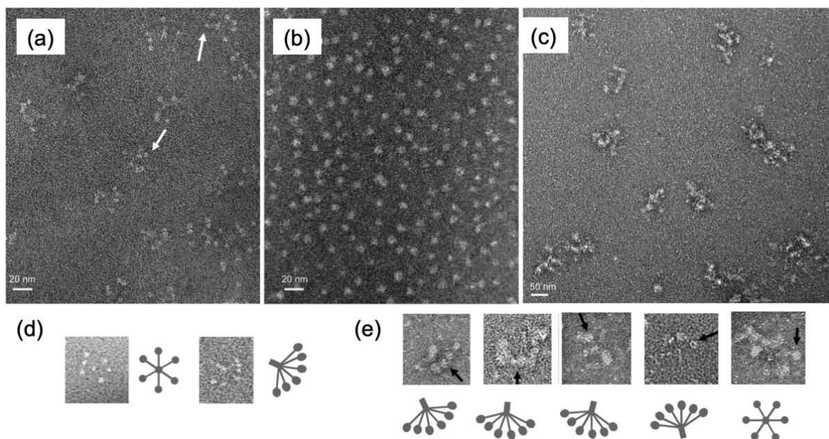
Figure 17. Transmission electron micrographs of C1q, \text{PrP} type II oligomers, and C1q- \text{PrP} complexes stained with 2% uranyl acetate or 1% ammonium molybdate. (a) C1q purified from human serum. White arrows point to globular head domains of C1q of ~4 nm. (b) \text{PrP} type II oligomers purified by SEC. The oligomers have a diameter of 5-8 nm. (c) A SEC fraction of C1q- \text{PrP} complex. (d) Top view and side view of C1q. (e) Side views and top view of purified C1q- \text{PrP} complexes. Black arrows point to examples of \text{PrP} bound to globular domains of C1q.
