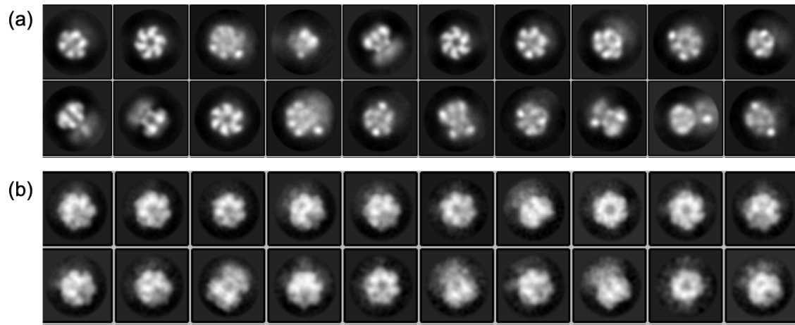
Figure 29. Two-dimensional class averages of the full-length D5 protein produced in E. Coli BL21 Star (DE3) (a) and in SF21 insect cells (b). ADP and Mg^{2+} ions have been added to both samples. The primase domain appears as diffuse density localized mainly on one side of the particle.
