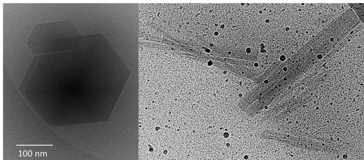
Figure 30. Different conditions yield different crystal forms of glucose isomerase crystals (samples from Dr. Van Driessche). Compact crystals are formed in one condition (left image). In another crystallization condition (right), monomers first form fibers, which then assemble to form elongated crystals.
