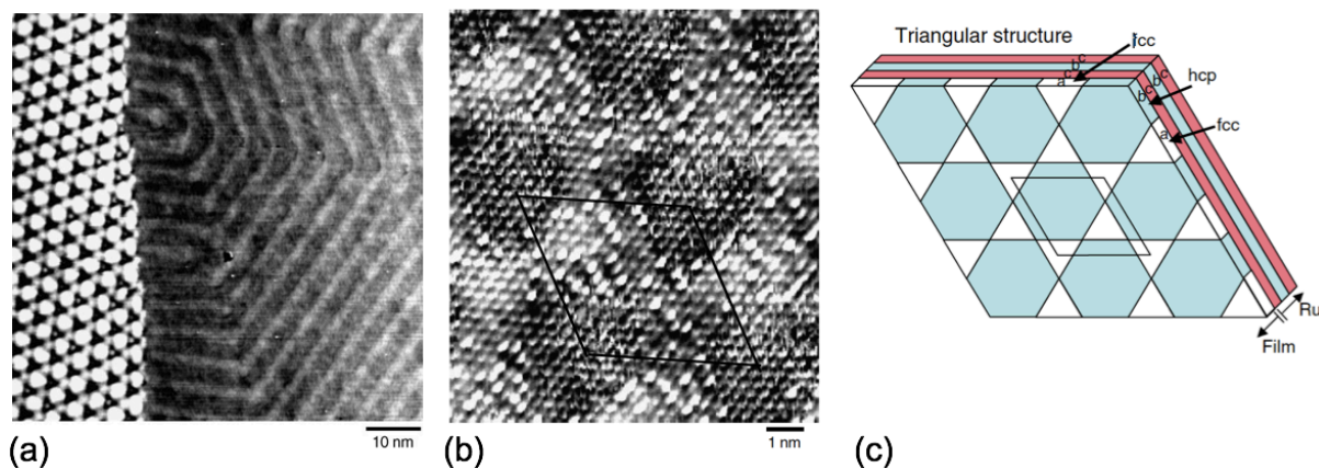
Figure 4. Triangular dislocation network of \text{Ag}_{0.5}\text{Au}_{0.5} alloy film. (a) Image of an alloy film with 1.3 ML average thickness showing the 2ML film with the triangular dislocation network on the left and a 1 ML film with the herringbone structure on the right across a monatomic Ru substrate step. (b) Atomically resolved STM image of the triangular dislocation network with a unit cell indicated. The second film layer form a hexagonal mesh free of threading dislocations. The Ag and Au atoms are distinguishable by their different contrast. The atom type that has a brighter contrast prefers one type of hollow site and the other atom type the other. (c) Schematic illustration of the stacking sequence of the 2 ML triangular dislocation structure. The letters indicate the stacking sequence relative to the Ru substrate. Shockley partial dislocations occur only at the first layer/substrate interface.
