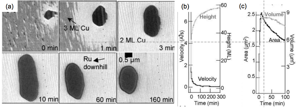
Figure 9. Post-deposition 3-dim growth of a Cu island on Ru(0001) at 600 °C. (a) Snapshots of a LEEM movie capturing the Cu island migrating 2.5 μm in 2.5 h down around 30 double atomic-layer Ru substrate steps, thereby increasing its height by nearly 60 ML. The dotted line marks the same Ru substrate step edge in each frame. (b) Speed of the island and its height as a function of time. (c) Volume and surface area of the island as a function of time. The volume increases initially as the island consumes the surrounding Cu, then stays constant while the island grows taller. The volume finally decreases as its atoms diffuse to thicker islands outside the field of view during ripening.
