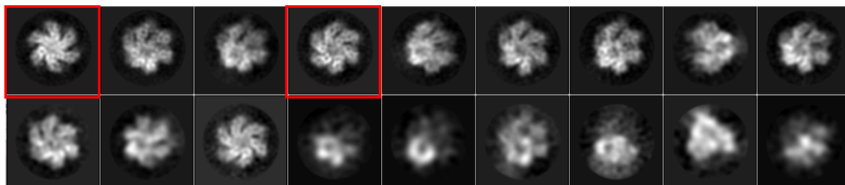
Figure 28. Two-dimensional class averages of cryo-electron microscopy images of D5 323-735 particles. Top views of different conformations of the proteins can be resolved (e.g. red boxes). No consistent 3-dim reconstruction could be obtained from the data set because of the lack of side views.
