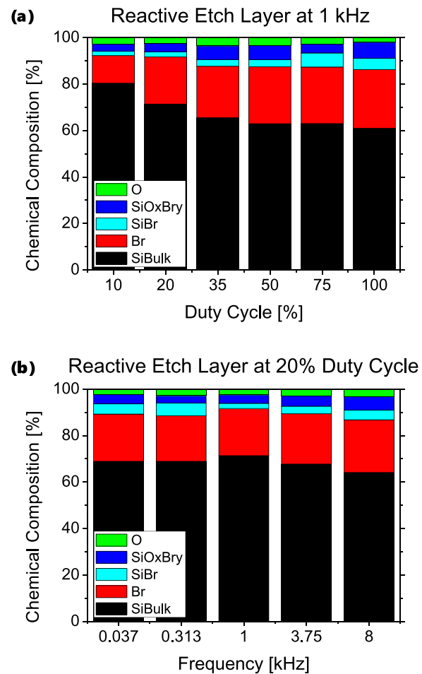
FIG. 7. (Color online) (a) Chemical composition of the XPS signal (at 46.25^\circ ) from the reactive etch layer for different duty cycles (at 1 kHz) and (b) frequencies (at 20% duty cycle).
