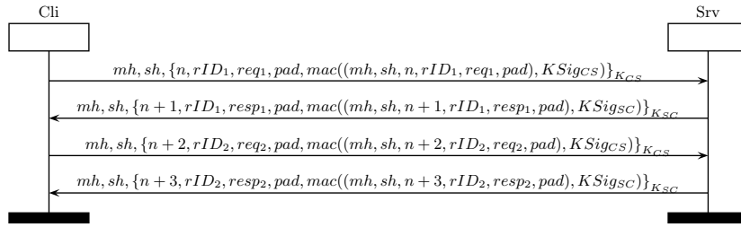
Figure 5: Two requests and responses in OPC-UA.
