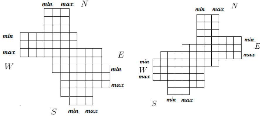
FIGURE 10. An element of the class \mathfrak{S}^{0,0} on the left and one of the class \mathfrak{S}'_{2L}{}^{0,0} on the right.
