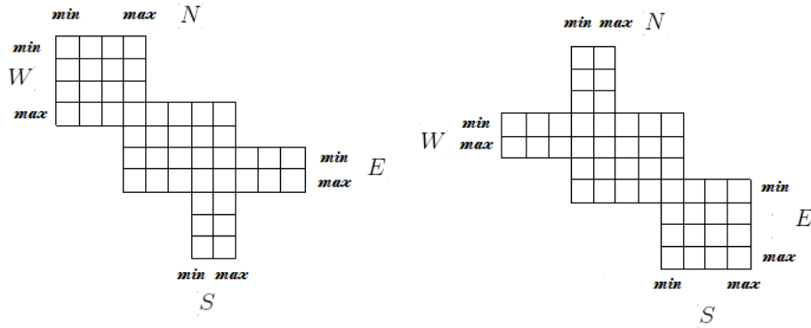
FIGURE 18. 2L-convex polyominoes in the classes \varphi_{2L}^0 (left) and \eta_{2L}^0 (right).
