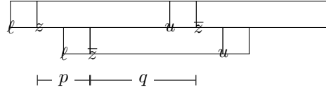
Figure 10: The word l\bar{z}u is factor of the word lzu\bar{z} .
